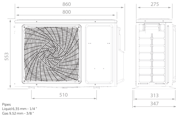
3U55S2SR5FA - 3U70S2SR5FA (3 couplings)
