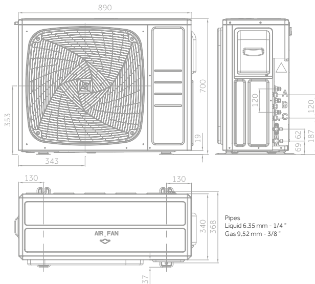
5U90S2SS5FA - 5U105S2SS5FA (5 couplings)
